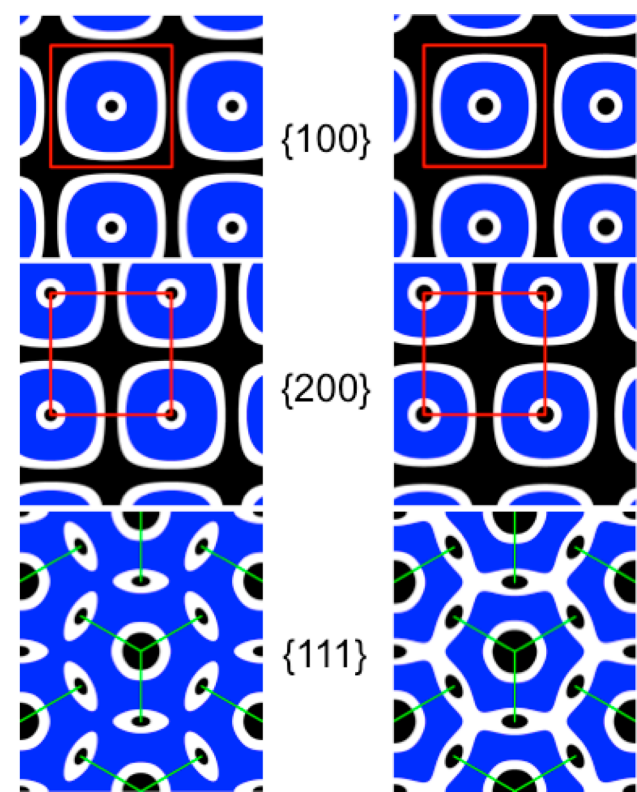
Figure 10. Simulated distribution of segregated zones in the cubic cell for complexes [P_2 C 1][DOS]_4 (left), and [P_3 C 1][DOS]_4 (right), within most important crystallographic families of planes (blue: mesogens + metallacycles sublayers; white: aliphatic strata; black: dendritic cores labyrinths; red frame: cubic lattice; green lines: edges to vertices from next plane).
