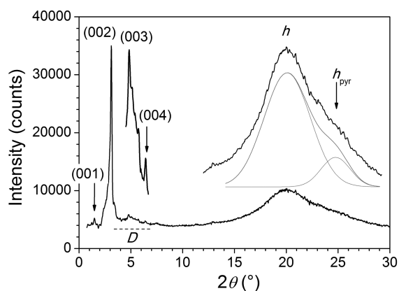
Figure 5. Representative SAXS patterns of P_3 at T = 80\text{ }^\circ\text{C} .
