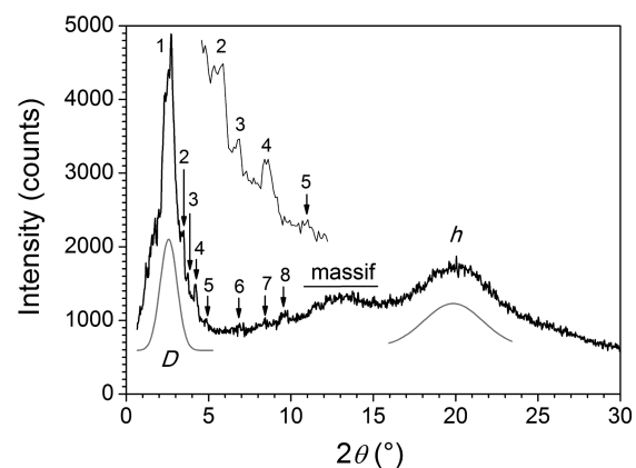
Figure 8. Representative SAXS patterns of [P_2 \subset 1][\text{DOS}]_4 at T = 80 ^\circ\text{C} .
