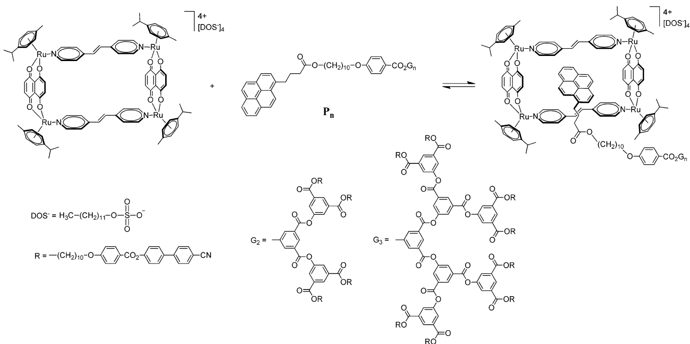
Scheme 2. Synthesis of the [\text{P}_n \subset 1][\text{DOS}]_4 Assemblies a
