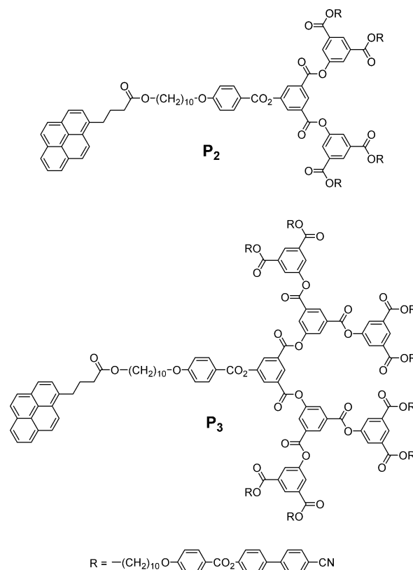
Figure 1. Structures of the second- and third-generation dendrimers \text{P}_2 and \text{P}_3 .
