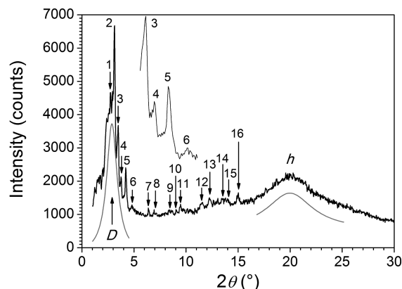
Figure 7. Representative SAXS patterns of [P_3 \subset 1][\text{DOS}]_4 at T = 80 ^\circ\text{C} .
